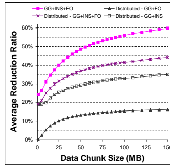
Fig. 12. Graph of the average reduction ratio of the centralized optimization (INS+FO) and three distributed optimizations (FO, INS, INS+FO) as a function of data chunk size for the greedy geographic tree GG.
