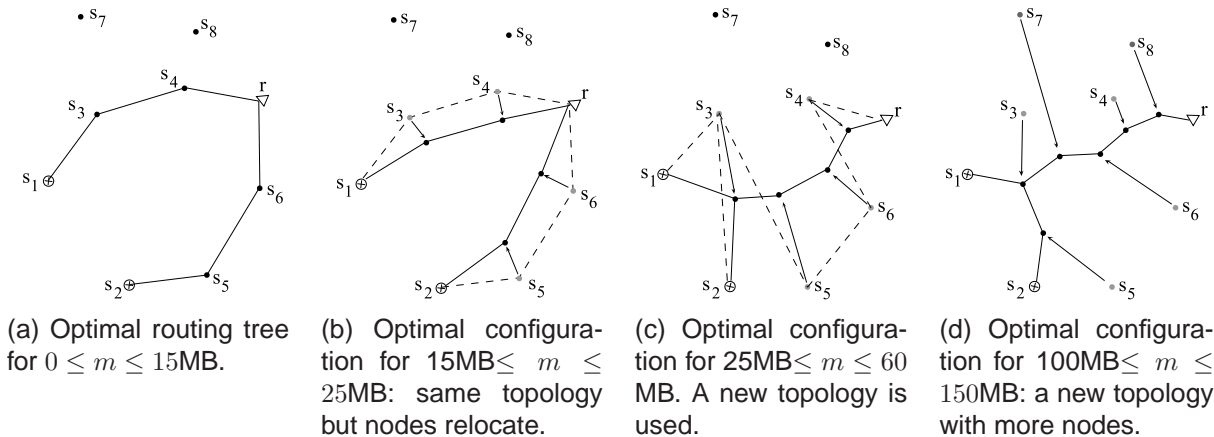
Fig. 2. Example of optimal configurations as a function of amount of data to be transferred. In each part, source nodes s_1 and s_2 must send m bits of data to the sink r . We consider m up to 150MB.
