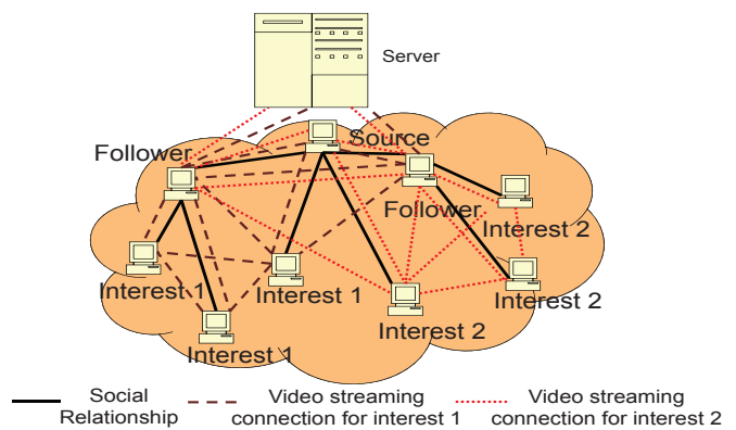
Fig. 13: Structure of SocialTube.
