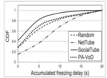
Fig. 23: CDF of accumulated freezing delay.
