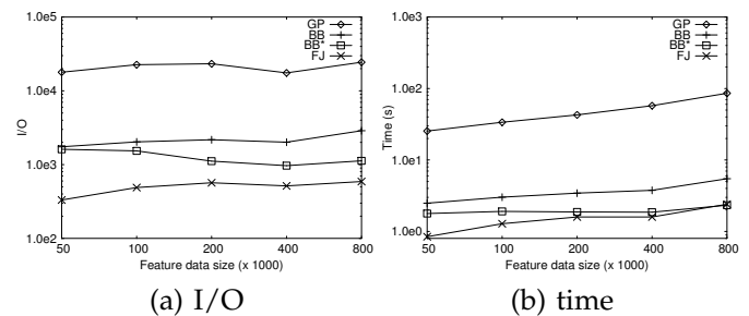
Fig. 10. Effect of |\mathcal{F}| , range scores
