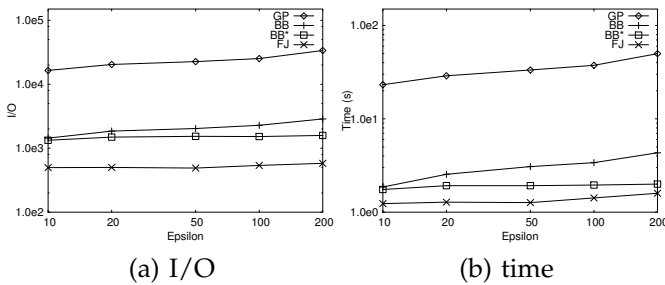
Fig. 13. Effect of \epsilon , range scores
