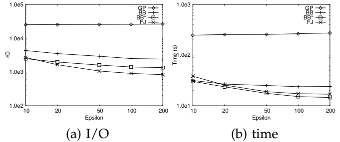
Fig. 16. Effect of \epsilon , influence scores
