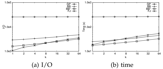
Fig. 15. Effect of k , influence scores
