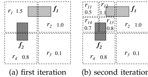
Fig. 7. Deriving upper bound of the influence score for FJ
