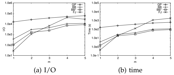
Fig. 14. Effect of m , influence scores
