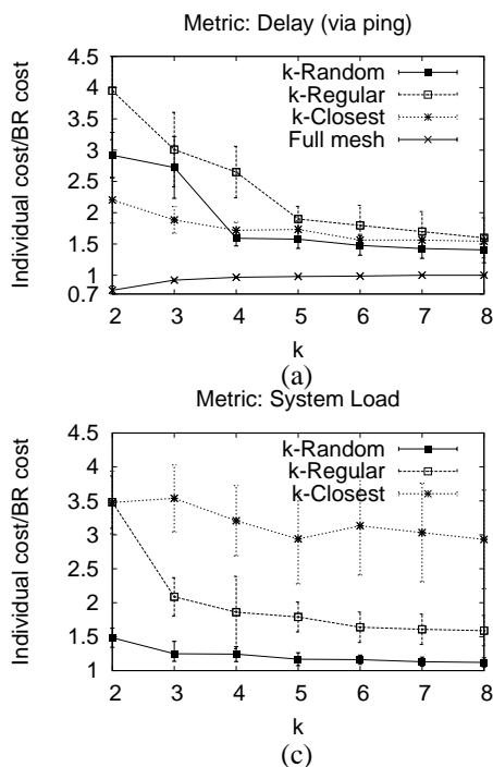
Fig. 4. Normalized individual costs and 95 th -percentile confidence intervals with respect to BR cost, under different metrics, of various neighbor selection strategies in a 50-node EGOIST overlay.
