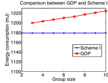
Fig. 7: Energy consumption per sensor node.
