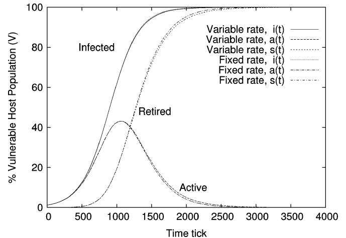
Fig. 8. Comparison of propagation curves for worms with variable- and fixed-rate of scanning. The simulation parameters used are N = 2^{23} , V = 2^{13} , and v = 100 . The value of r is a constant five scans per time tick for the fixed-rate scanning worm, and the other having variable rates with the Gaussian distribution and a mean value of 5 per time tick.
