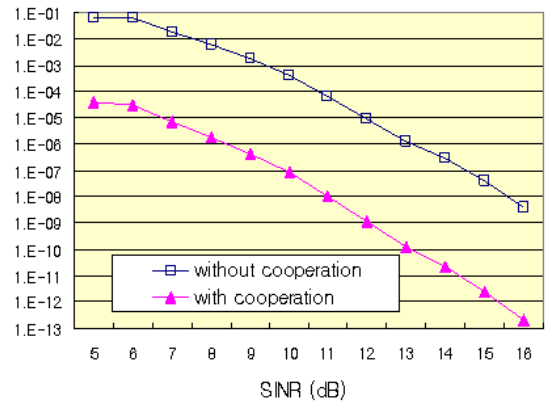
(a) BER versus SINR
