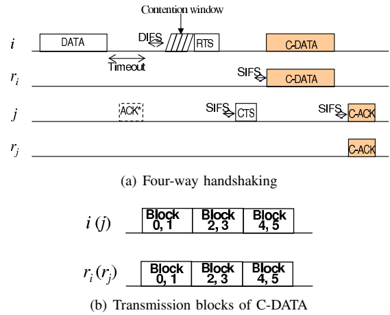
Fig. 4. CD-MAC with partners r_i and r_j on a weak link ( i, j ). (RTS is normally not used in CD-MAC but it is employed in Fig. (a) because the preceding communication failed. The DATA frame in this figure consists of 6 blocks as in Fig. 3.)
