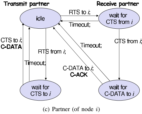
Fig. 5. State transition diagrams for a sender, a receiver and a partner. (Figure (c) shows the state transitions of a transmit partner as well as a receive partner.)
