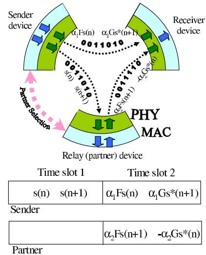
Fig. 1. Cooperative communication using distributed space-time coding scheme based on single channel model. (* denotes conjugation and two real coefficients \alpha_1 and \alpha_2 are related to each other by \alpha_1^2 + \alpha_2^2 = 1 [8].)
