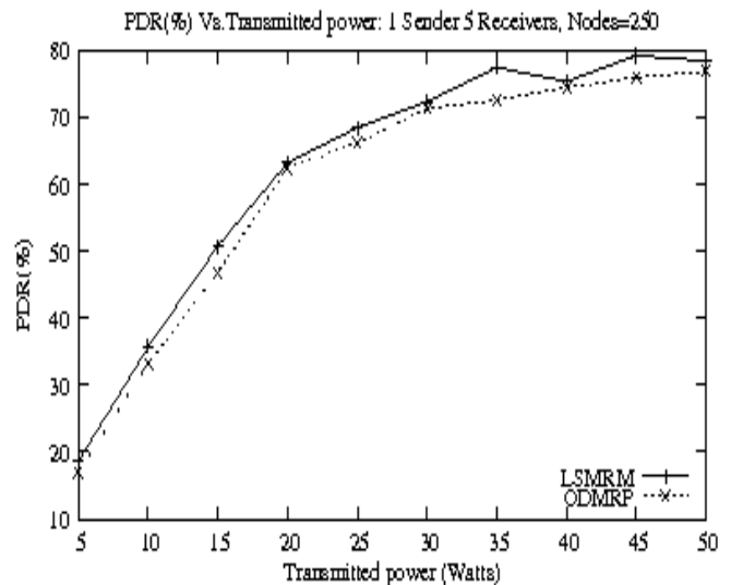
Fig. 9. PDR Vs. Transmitted power (nodes=250)
